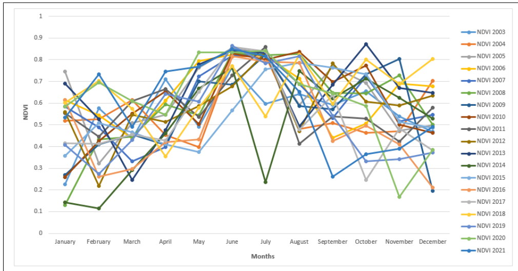
Figure 3.4: NDVI time series monthly for each year
