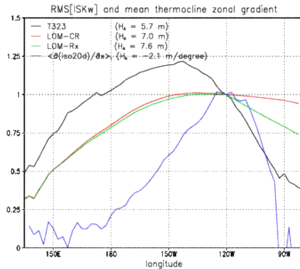
Figure 7. RMS of ISKw for T323 (black line), LOM-CR (red line), and LOM-Rx (green line). The blue line shows the temporal mean of the zonal gradient of the 20°C isotherm (thermocline) depth from T323. Values are adimensionalized by their respective values at 120°W (indicated in the upper left corner as H_k ).
