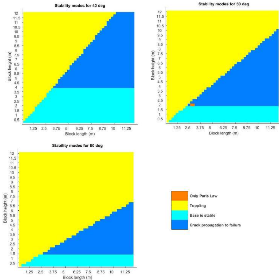
FIGURE 5.1: Results of the analysis performed. Three different angles, for 40°, 50° and 60°. Four zones are observed in the graph, depending on the blocks characteristics, it will be plotted in a specific zone. These zones include: the base provides stability, the crack is propagating to failure, the block should topple and the crack expands but only Paris law dominates the expansion.
