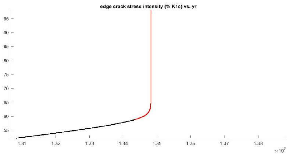
FIGURE 5.5: Zoom from the figure 5.3 for the transition Paris law - Charles law for the edge crack stress intensity
