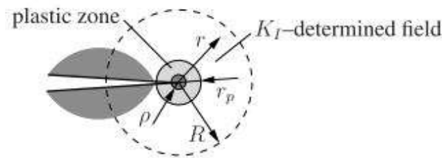
FIGURE 2.4: The figure shows the area of influence of K_I . (Gross and Seelig, 2011)
