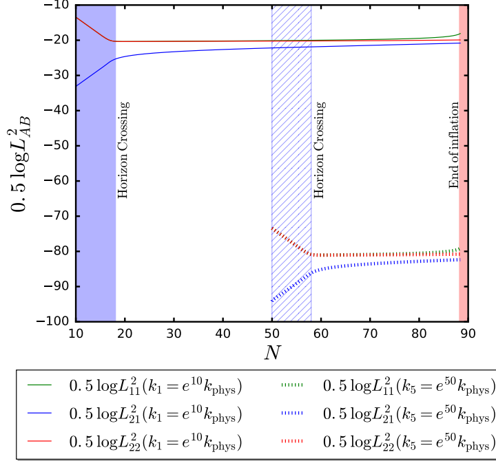
Figure 3.9: Evolution of two real Cholesky modes inserted at N \equiv \ln a = 10 and N = 50 . We detect the suppression of oscillations before crossing the horizon (at \ell = 1/H ).
