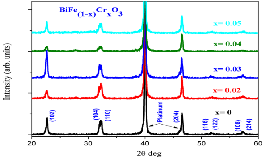
Figure 5.3 X-ray diffraction pattern for BiFeO 3 and BiFe 1-x Cr x O 3 thin films.
