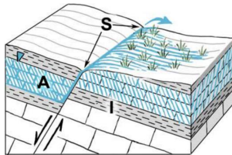
Fig. 1. Helocrene. Modified from Meinzer (1923). Springer et al., 2008.
